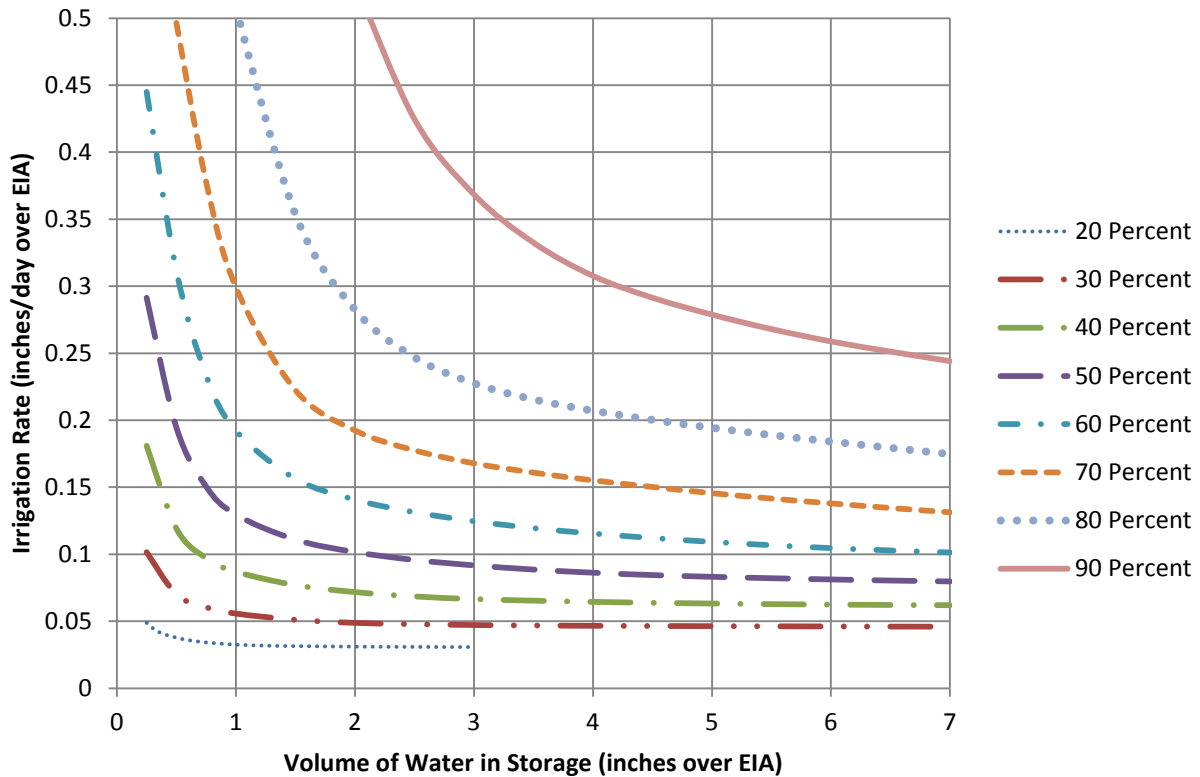
Figure 3.3-1 Rate Efficiency Volume (REV) Curve for Designing a Harvesting System for Sarasota County Florida
