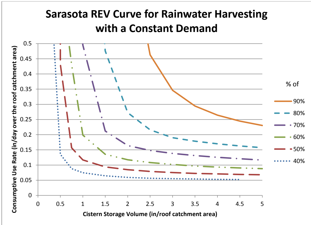
Figure 3.5-4 REV Curves for Rainwater Harvesting in Sarasota, FL with a Constant Daily Demand
