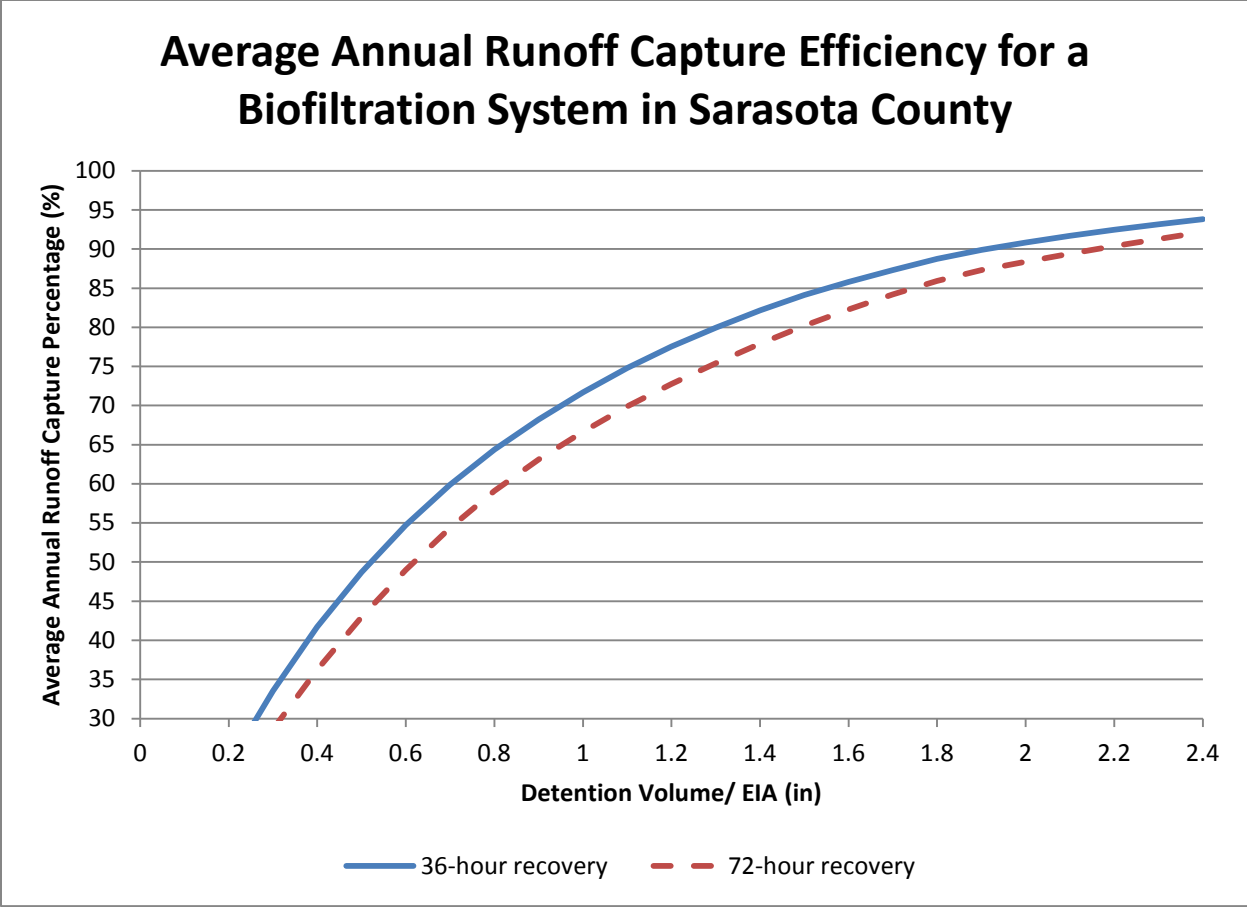
Figure 3.6-4 Biofiltration System in Sarasota County
